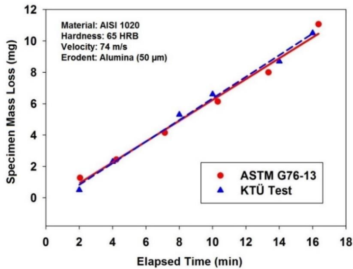
Figure 3. Comparison of erosion tests on AISI 1020 with ASTM G76-13 for calibration of solid particle erosion test system
